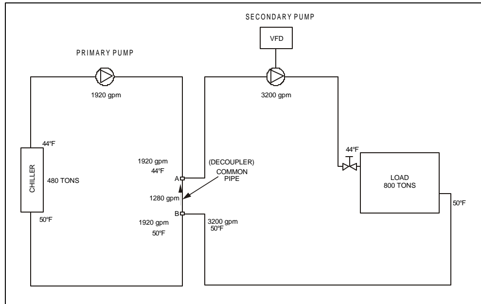
Figure 13, Primary/Secondary Loop at Low Delta-T
