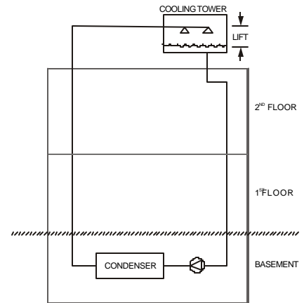
Figure 3, Open Loop
