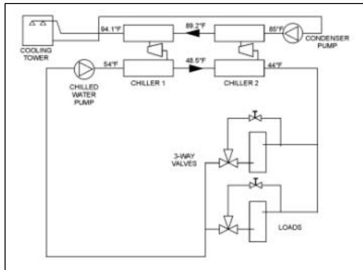
Figure 10, Series Chillers
